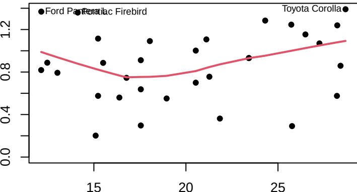
Scale-Location
